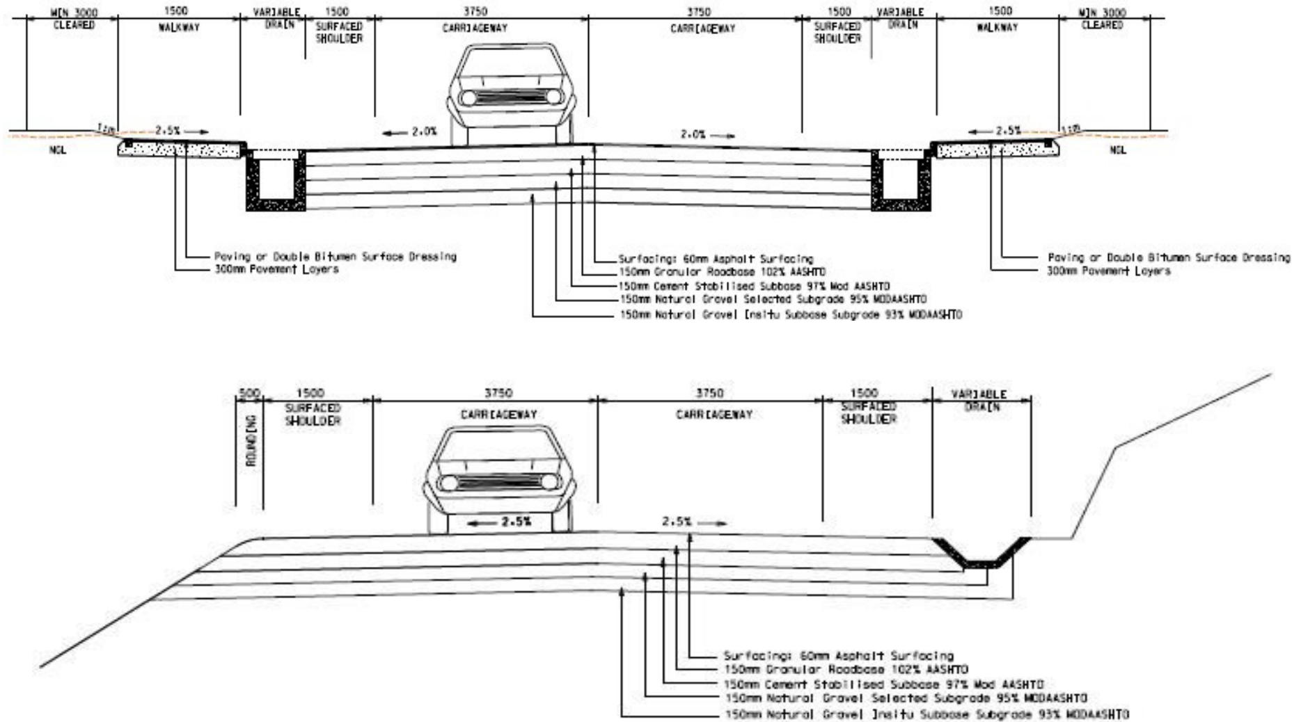
Figure 3-3: Typical cross section in (a) towns/villages and (b) rural areas (Source: Final Conceptual Design Report, January 2020)
